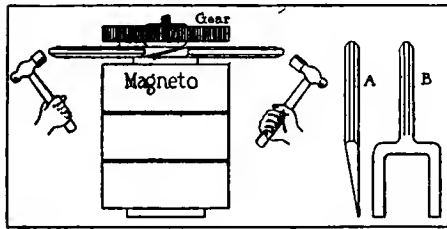
Fig. 1.—Removing magneto gear and the special tools to use
